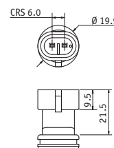
2 WAY PACKARD METRI-PAK 150 SERIES CONNECTOR.
